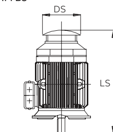
Protective roof, variant code 005
