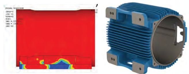
Figure 4 - Solid feet
